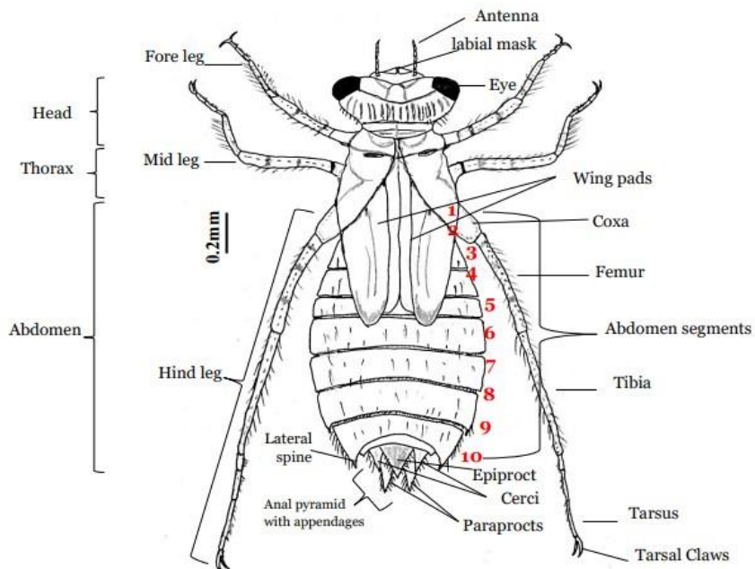
Figure 1: General morphological features of an Anisoptera naiads ( Crocothemis servilia )
