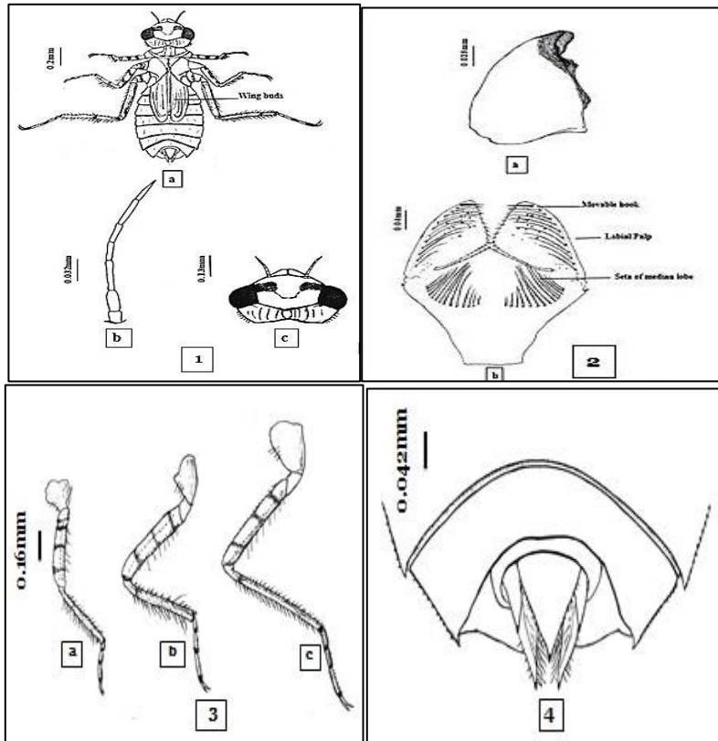
Plate 2: Crocothemis erythraea naiad, 1- General shape: a- Body, b- Antenna, c- Head; 2- Parts of the mouth: a- Mandible, b- Labium, c- Enlarged part for movable hook; 3- Legs: a- fore, b- mid, c- hind; 4- Dorsal view of anal appendages.
