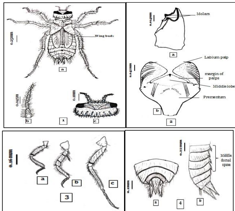
Plate 6: Orthetrum sabina naiid, 1- General shape: a- Body, b- antenna, c- Head; 2- Parts of the mouth: a- Mandible, b- Labium; 3- Legs: a- Fore, b- Mid, c- Hind; 4- Anal appendages: a- Lateral view, b- Dorsal view.
