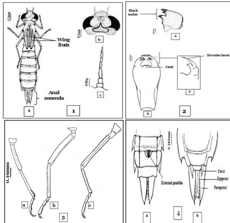
Plate 1: Anax parthenope naiad, 1- General shape: a- Body, b- Head, c- Antenna; 2- Parts of the mouth: a- Mandible, b- Labium, c- Enlarged part for movable hook; 3- Legs: a- Fore, b- Mid, c- Hind; 4- Anal appendages: a- Dorsal view, b- Ventral view.
