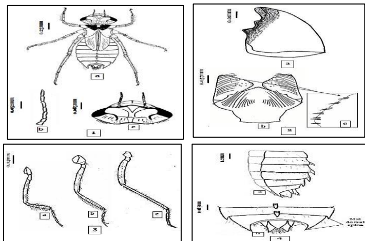
Plate 7: Selysiothermis nigra naiad, 1- General shape: a- Body, b- Antenna, c- Head; 2- Mouth parts: a- Mandible, b- Labium, c- Enlarged rim part of the interior of the labial palps, 3- Legs: a- Fore, b- Mid, c- Hind; 4- Abdomen and anal appendages: a- Lateral view, b- Dorsal view.
